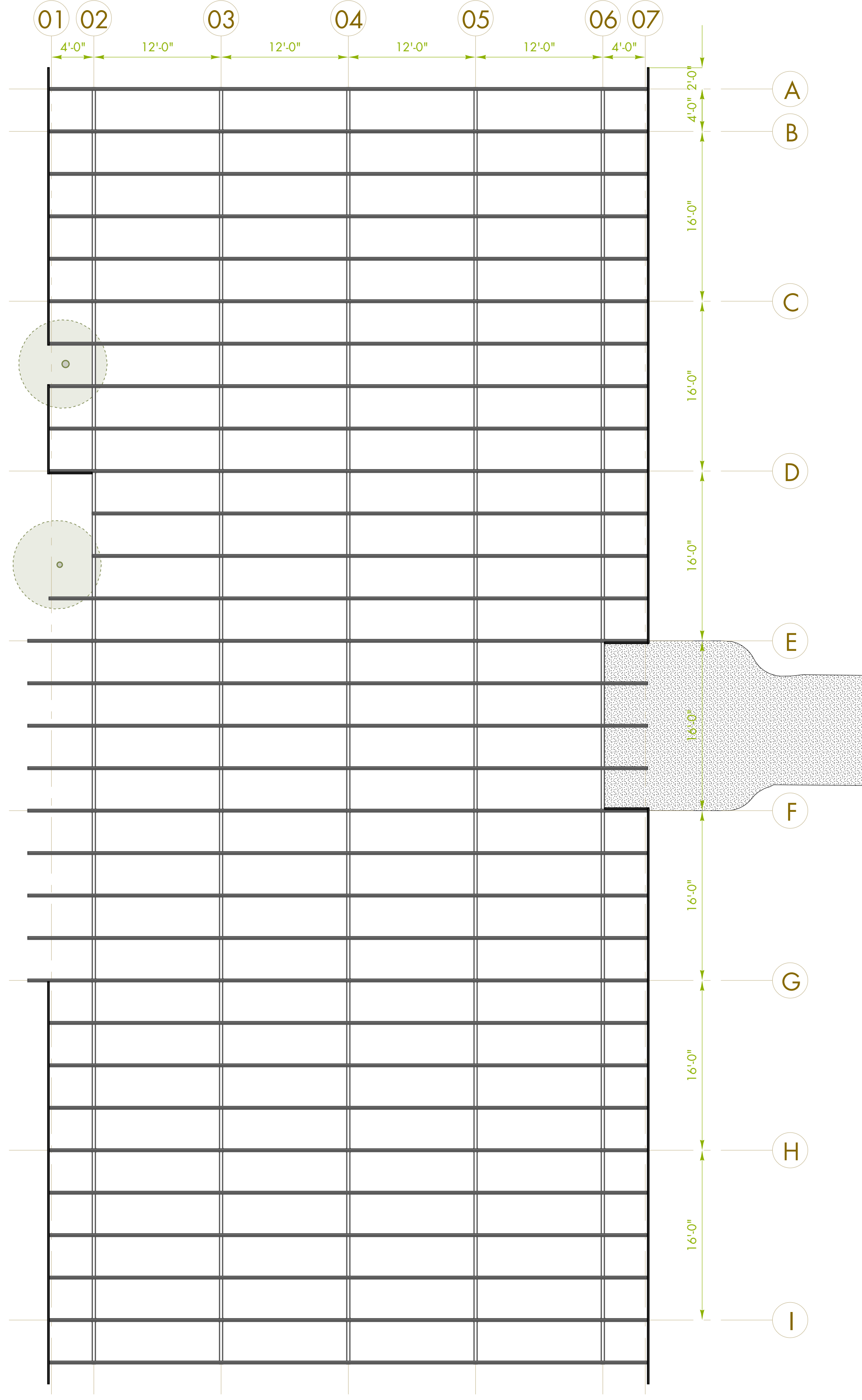
2 FRAMING PLAN 1/8" = 1'-0"
